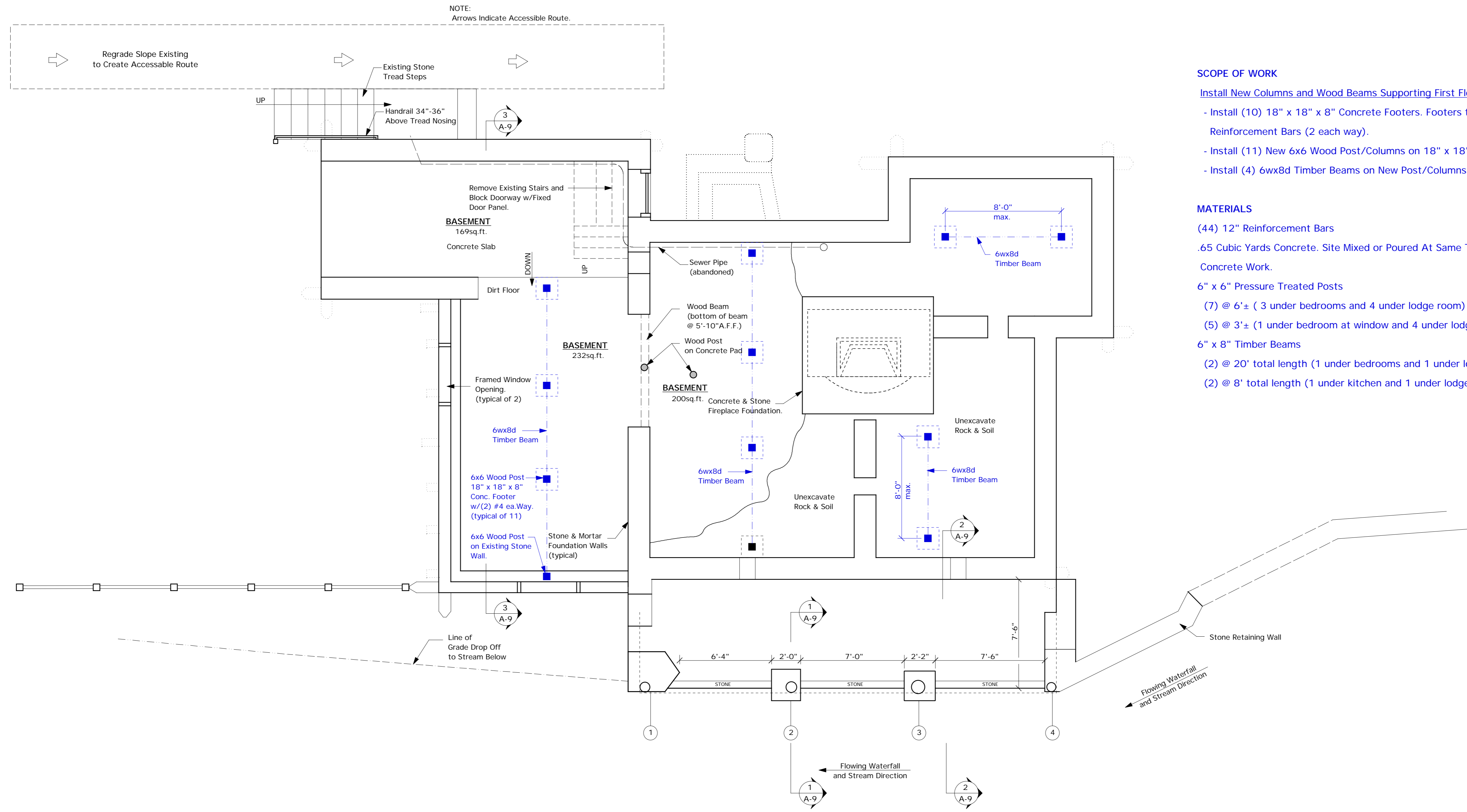
BASEMENT/FOUNDATION PLAN SCALE: 1/4" = 1'-0"
