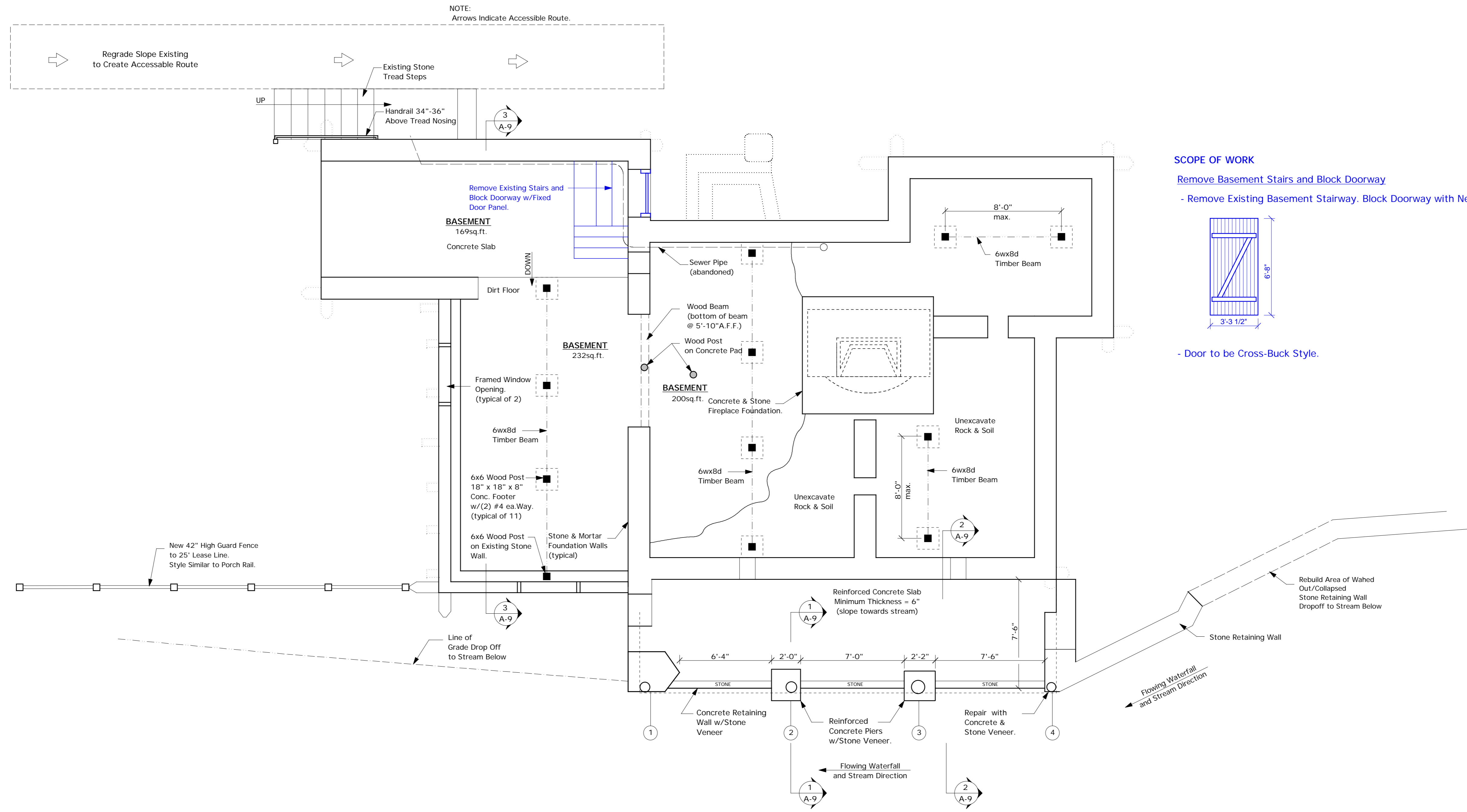
BASEMENT/FOUNDATION PLAN
